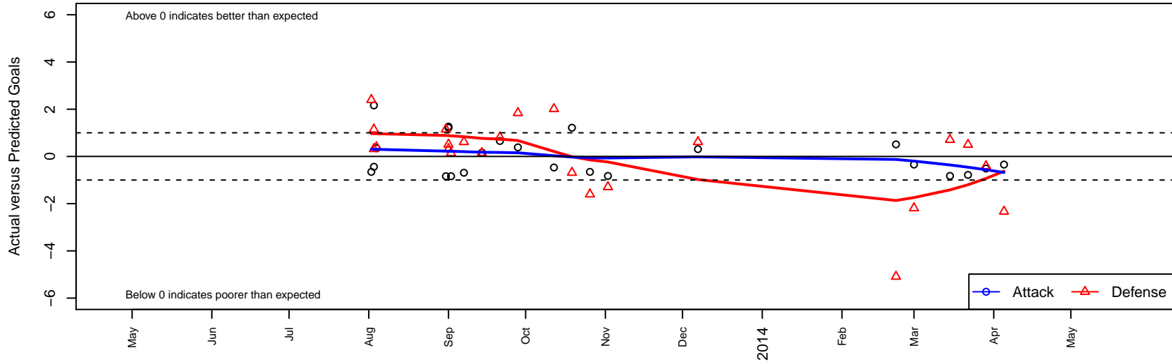
Kent United Black G01 Dots are actual minus expected GF (blue circles) and GA (red triangles). Blue line is smoothed change in attack strength. Red is smoothed change in defense strength.
